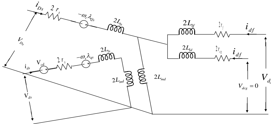
Figure 4: D-Axis equivalent circuit of the hybrid synchronous machine
