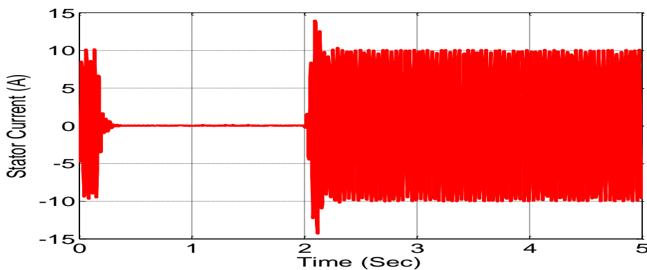
Figure 8: Control winding stator current (phase a) of the hybrid synchronous machine
