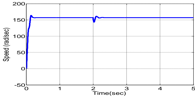
Figure 4: Speed-time characteristics of the machine
